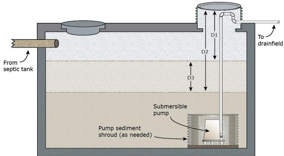
Pump Chamber Drawing
